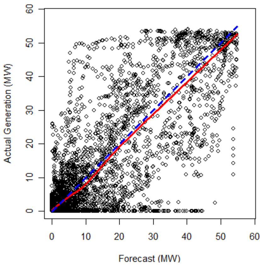
Figure 18 - White Hill eight hour energy
