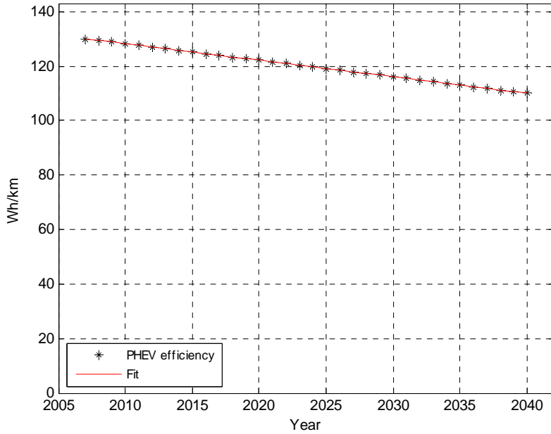
PHEV efficiency forecast
