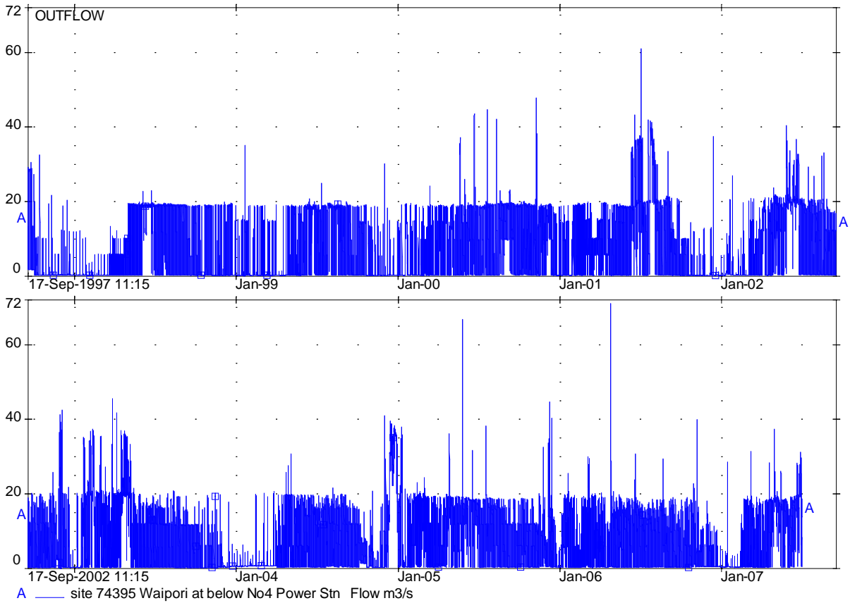
Figure 2.1: Waipori at Below No 4 Power Station flow
