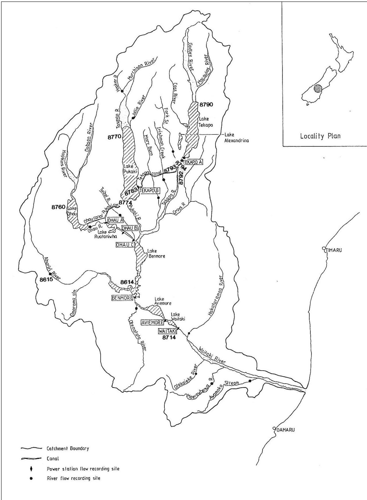
Figure 3.2: Waitaki hydro scheme
