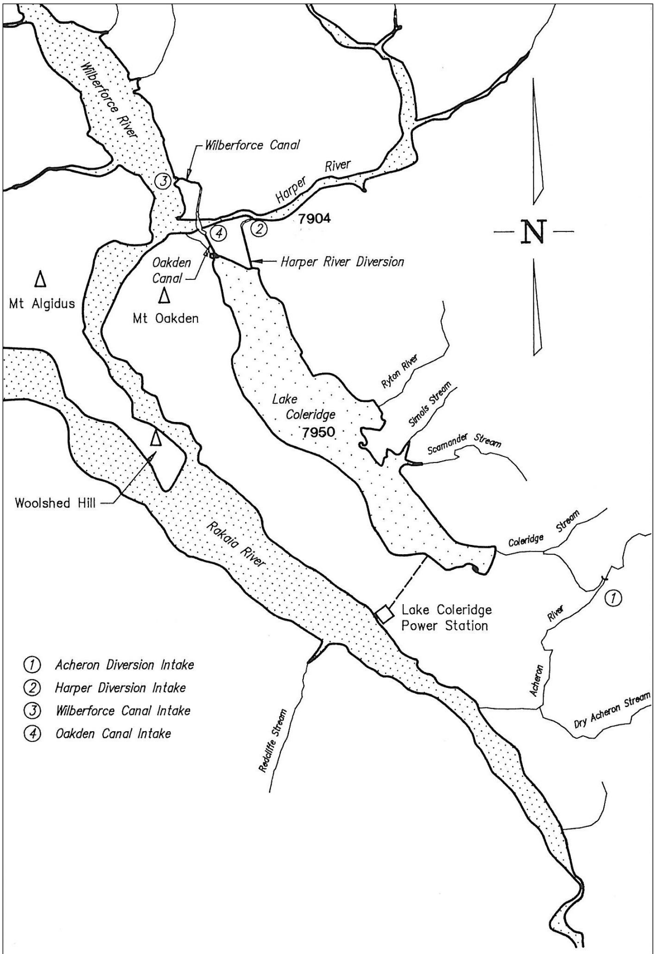
Figure 3.8: Layout of Coleridge Power Scheme
