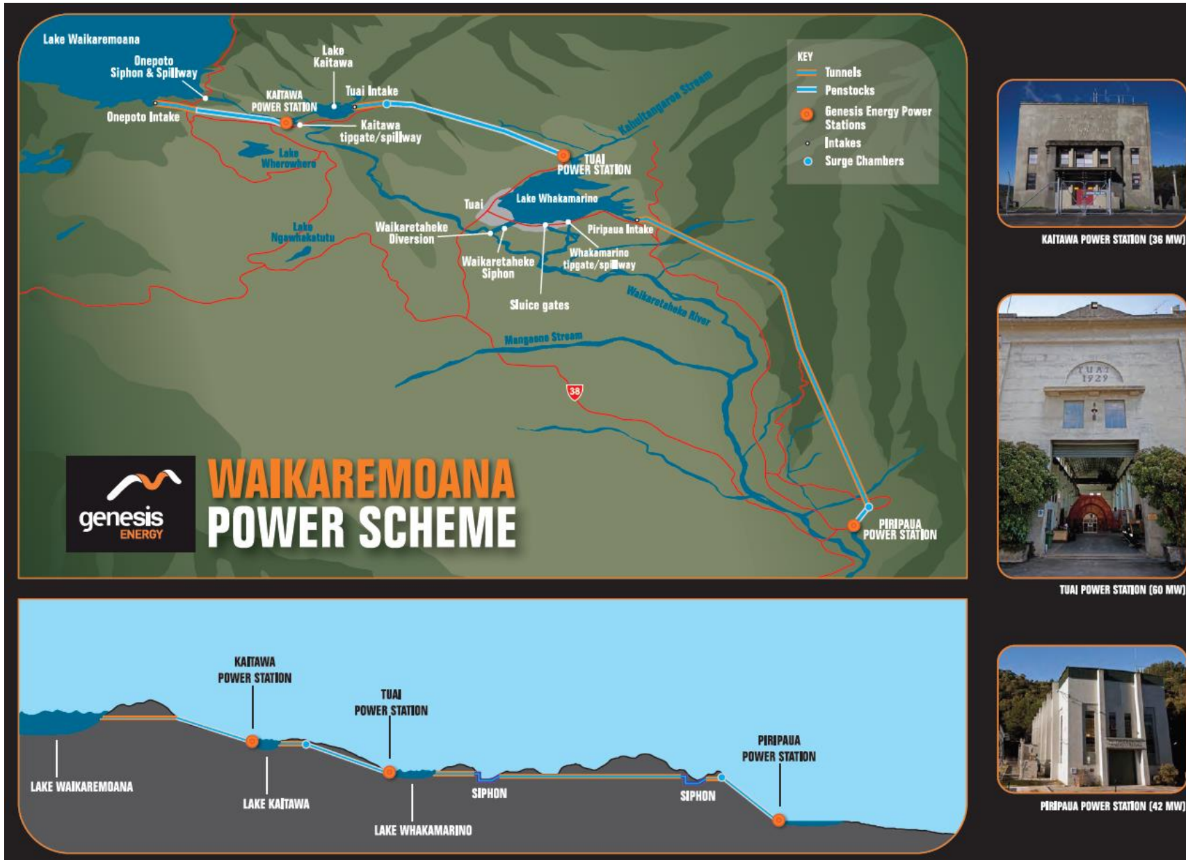
Figure 2.4: Schematic flow diagram for Waikaremoana (from genesisenergy.co.nz)
