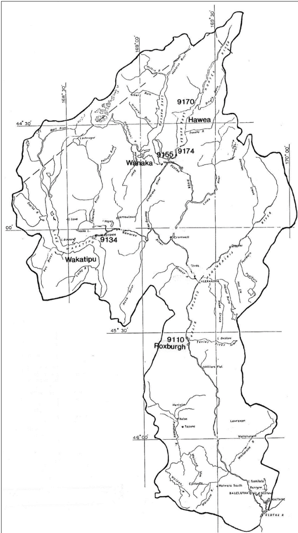
Figure 3.6: Clutha catchment
