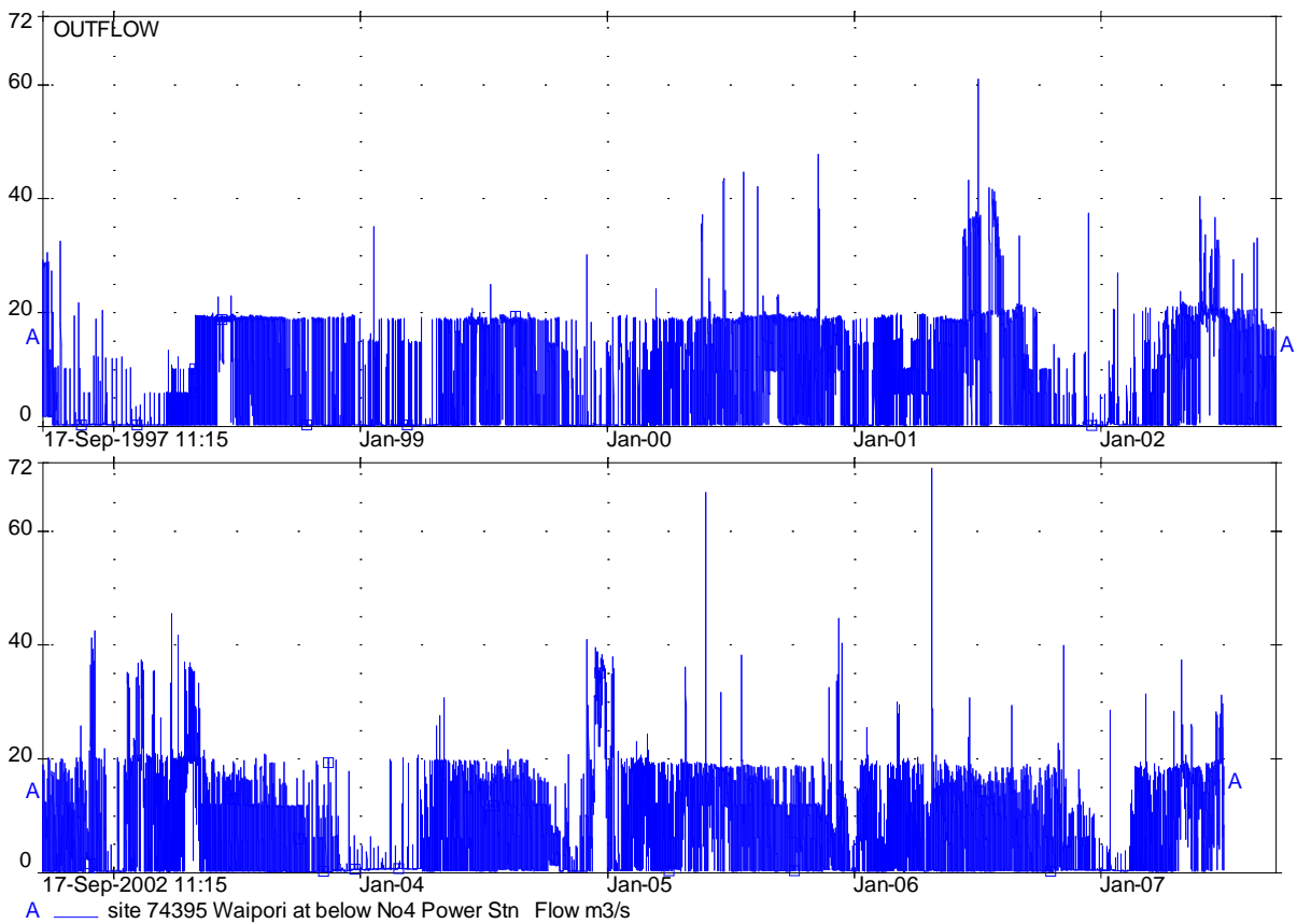
Figure 2.1: Waipori at Below No 4 Power Station flow
