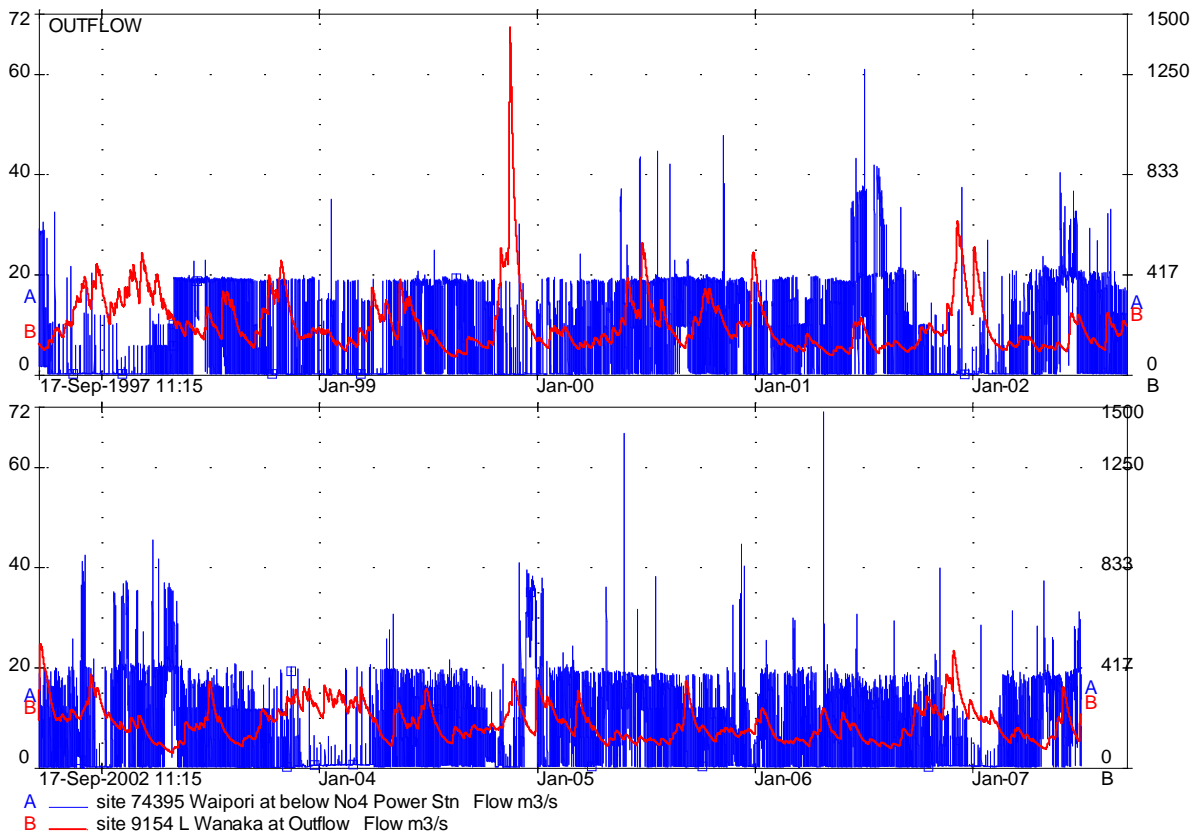
Figure 2.2: Waipori at Below No 4 Power Station flow compared with Lake Wanaka Outflow
