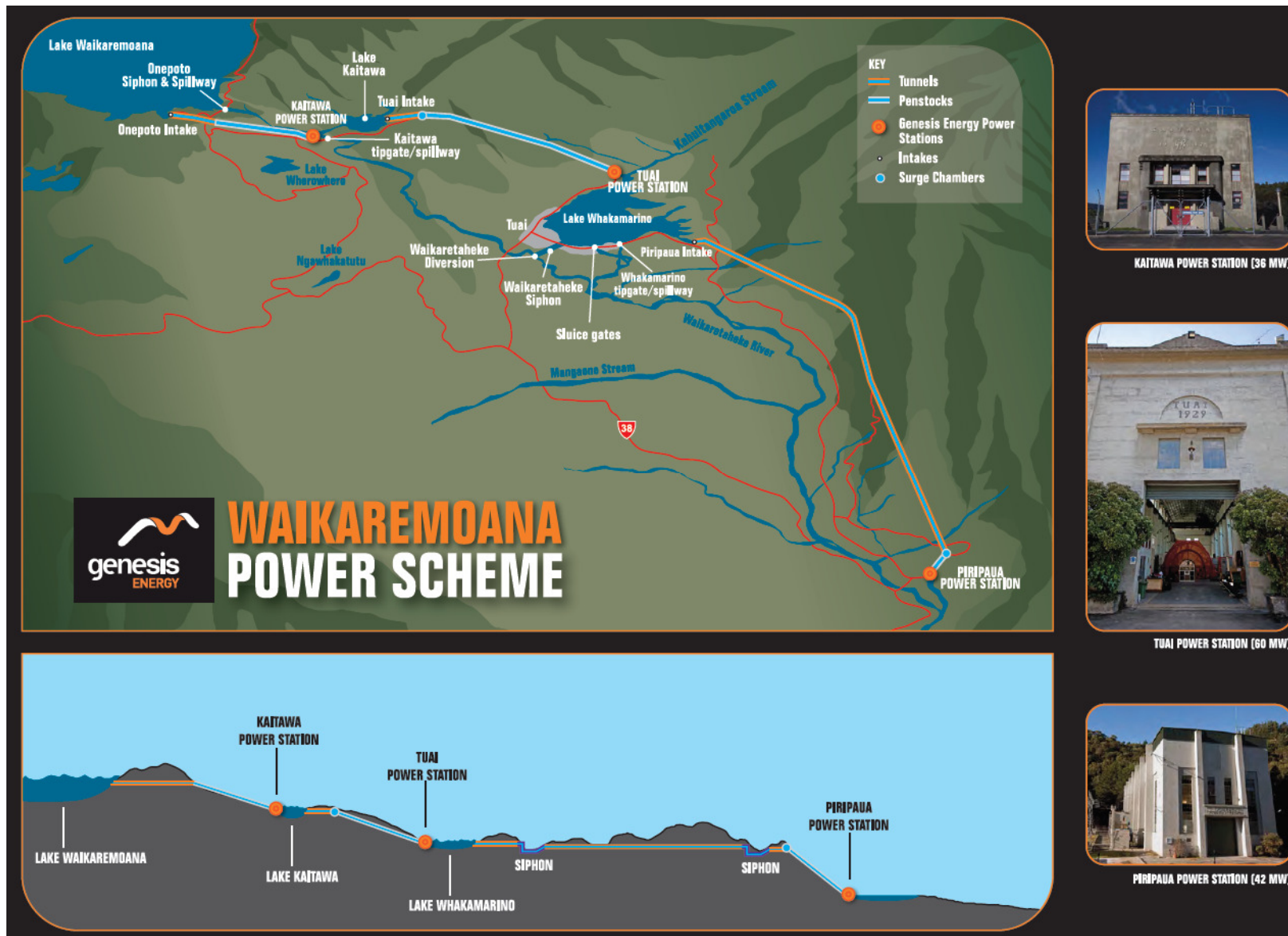
Figure 2.4: Schematic flow diagram for Waikaremoana (from genesisenenergy.co.nz )
