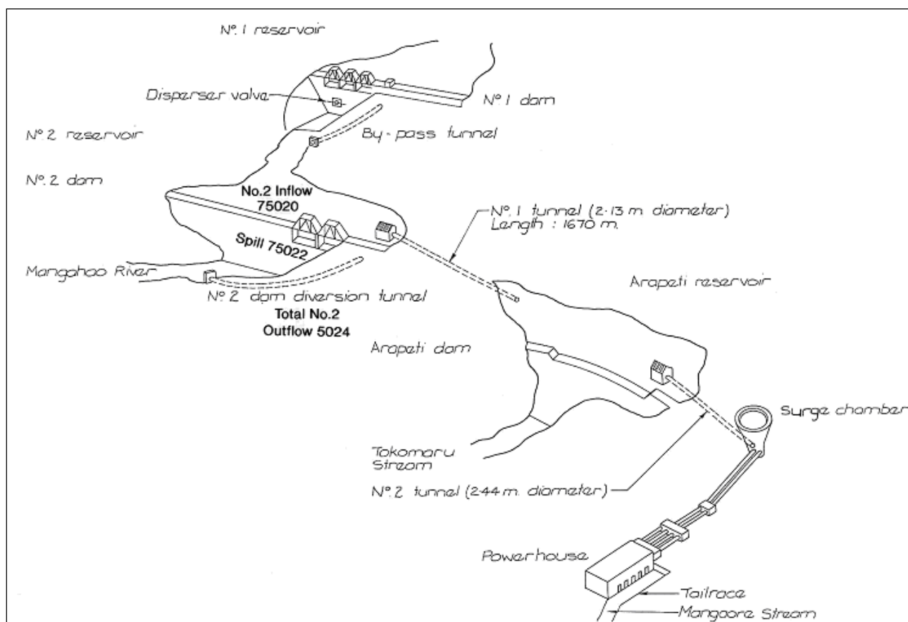
Figure 2.7: Schematic layout of Mangahao Power Scheme
