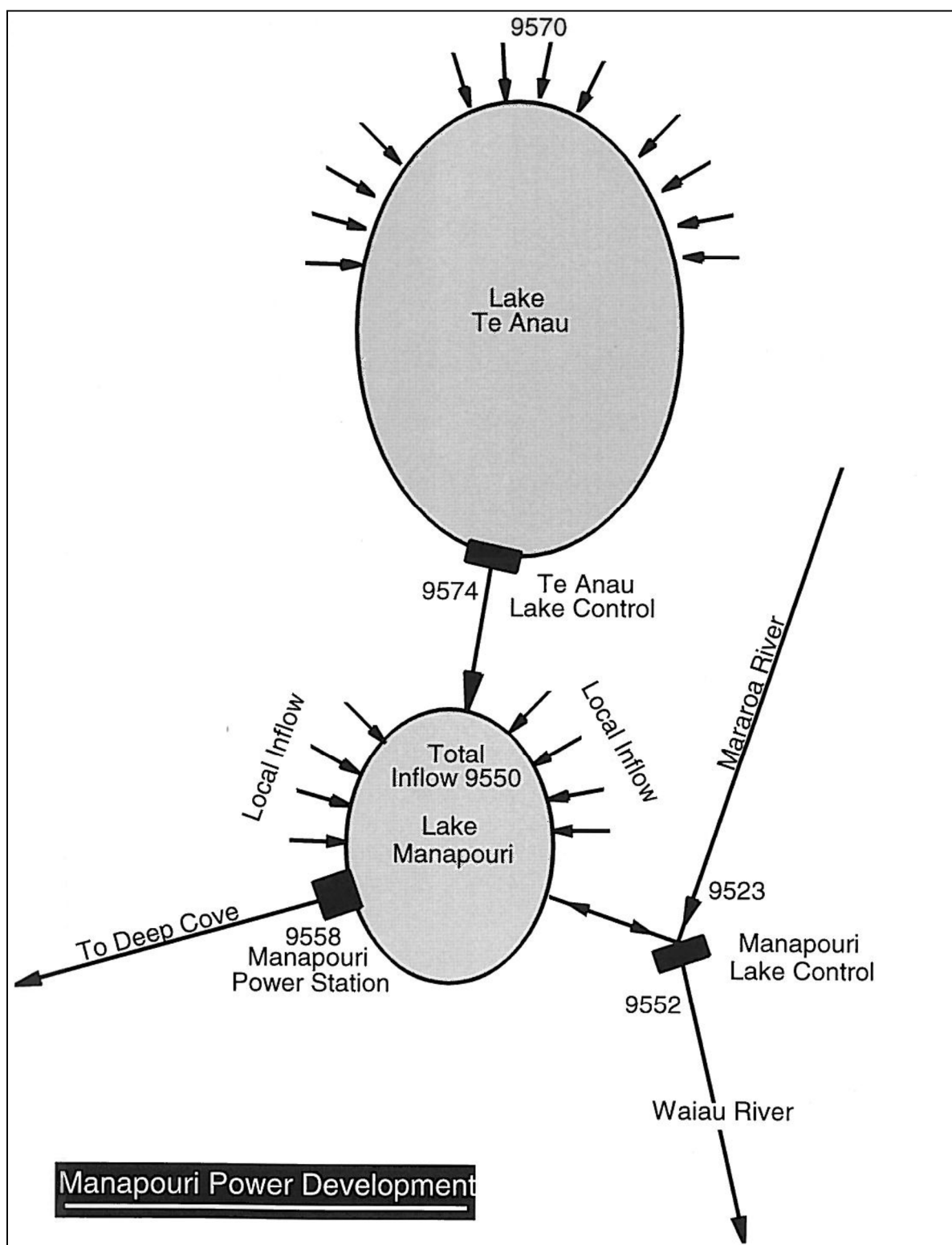
Figure 3.3: Schematic layout of the Manapouri Power Development
