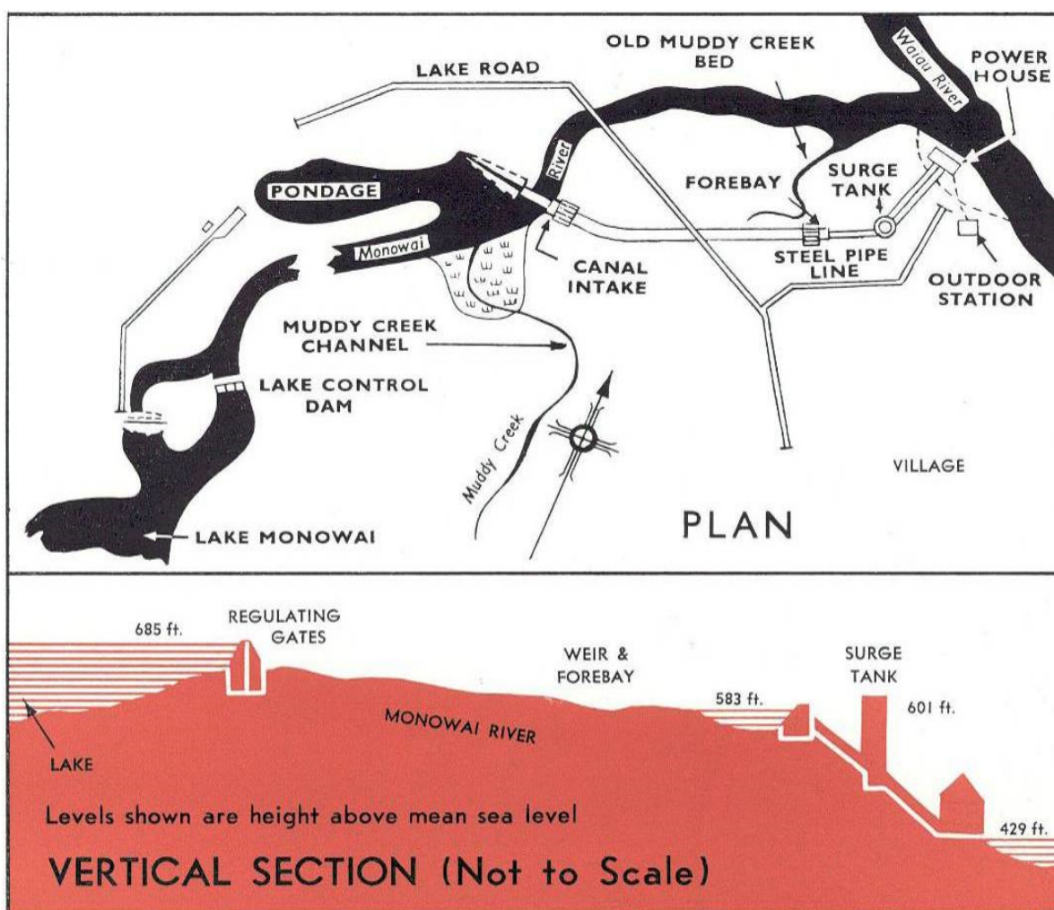
Figure 3.4: Monowai Power Development plan (original development)
