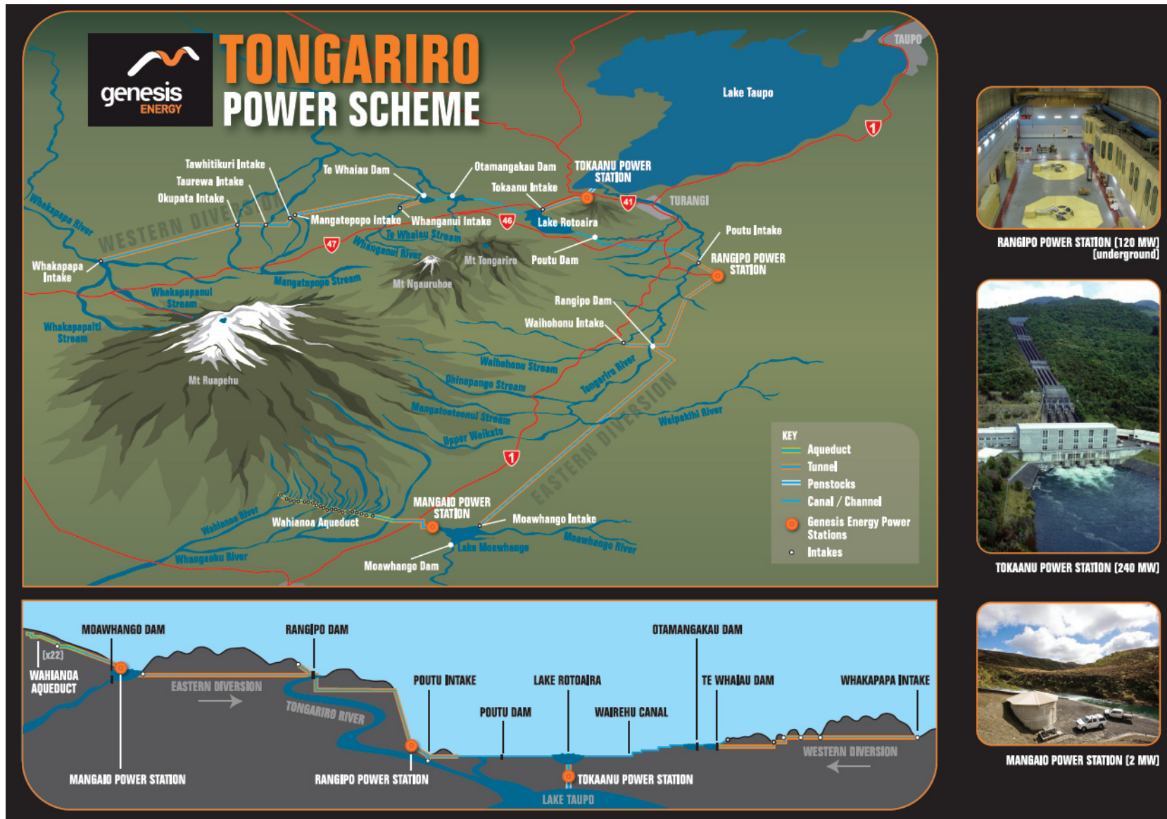
Figure 2.2: Schematic layout of the Tongariro Power Development and its various components (from genesisenergy.co.nz )
