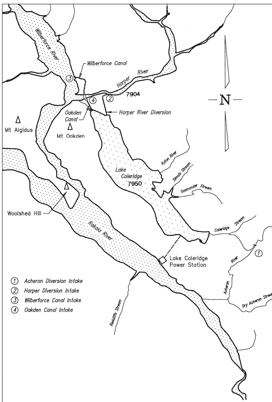
Figure 3.7: Layout of Coleridge Power Scheme
